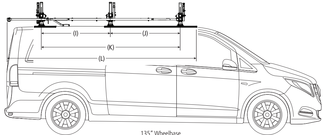
135" Wheelbase
