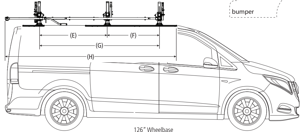
126" Wheelbase
