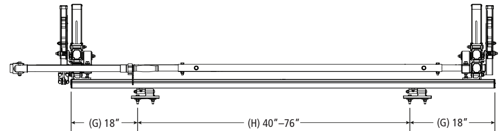
Alternate Installation
