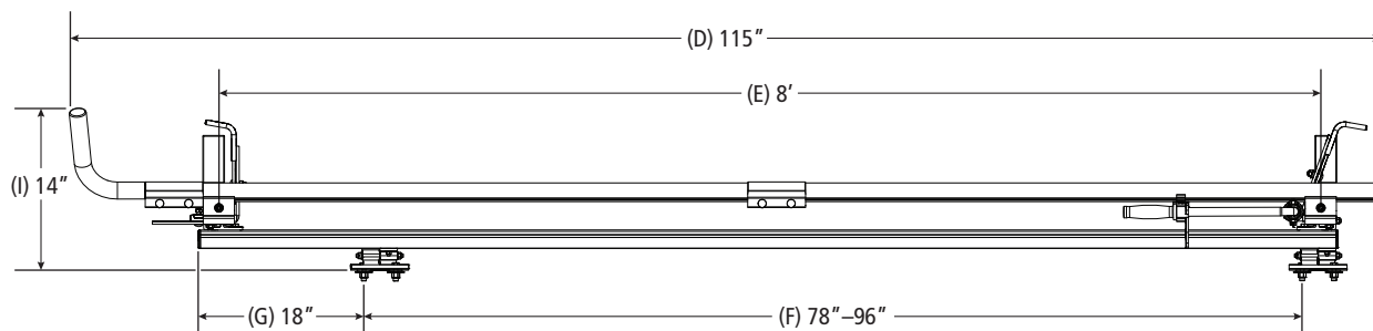
Typical Installation
