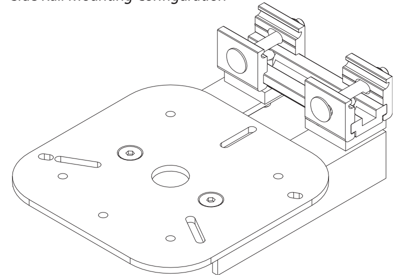
Side Rail Mounting Configuration
